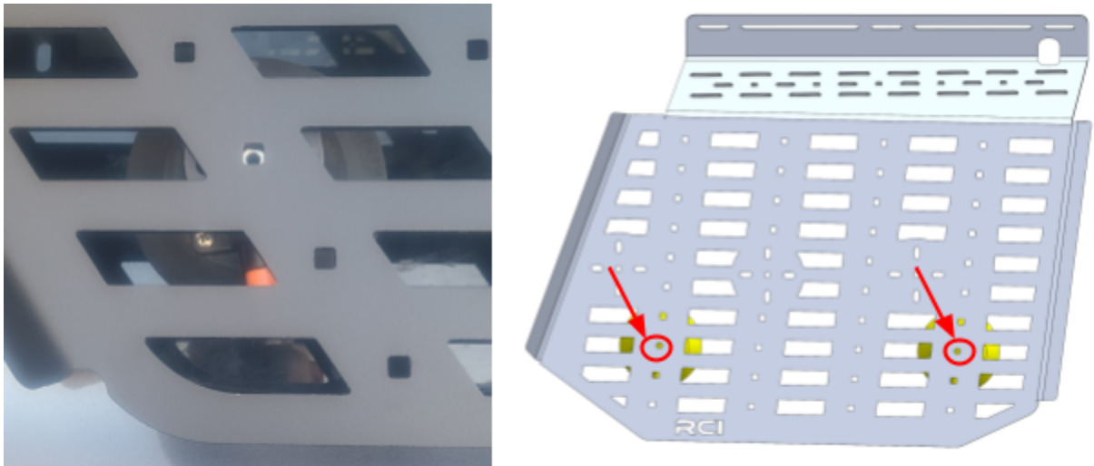
Figure 2: Suction Cup Alignment
