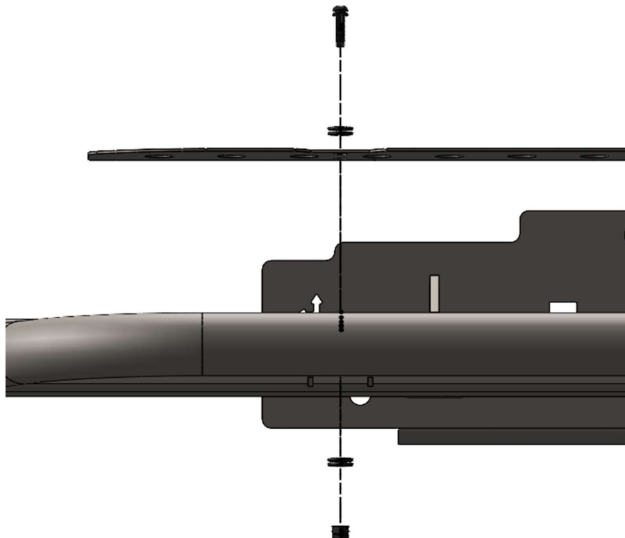
Figure 10: Hardware orientation.
