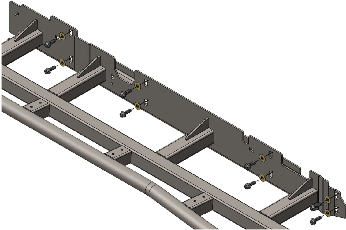
Figure 5: M10x30mm mounting locations.
