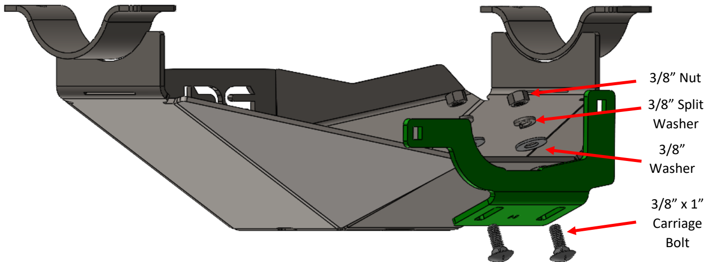
Figure 2: Lower Pinion Clamp Installation
