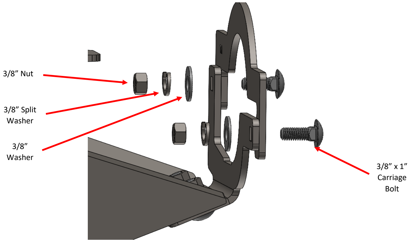
Figure 5: Pinion Clamp Hardware
