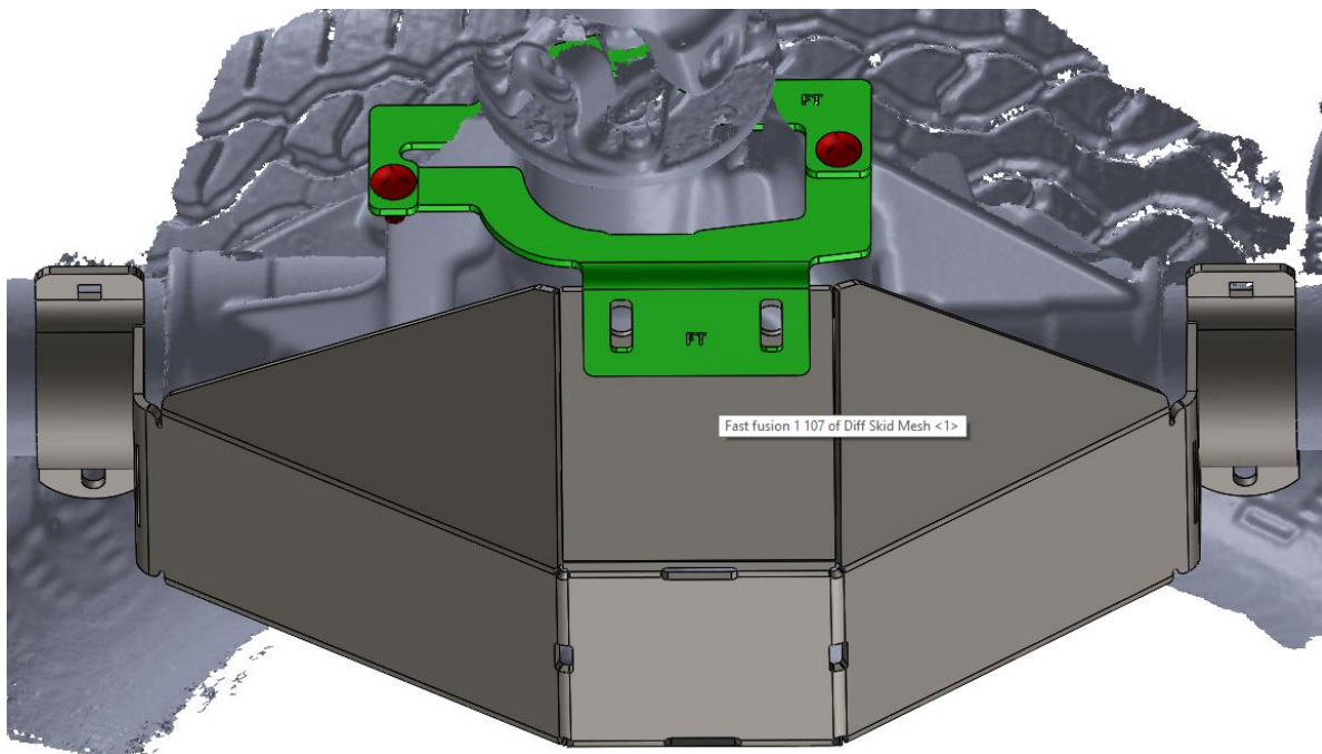
Figure 4: Upper Pinion Clamp Installation
